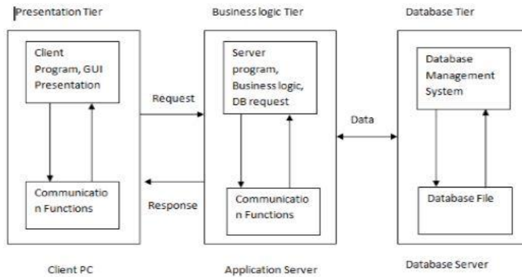
Figure 1.1: 3-tier architecture
