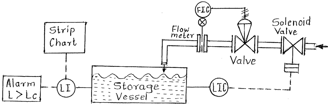
Figure Level control system with alarm.
