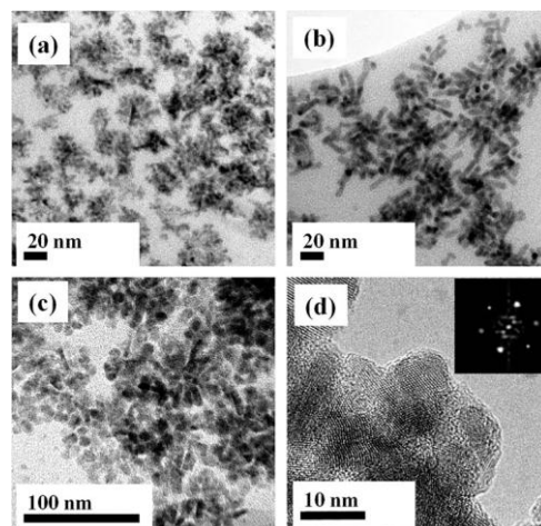
TEM images of CdS nanoparticles synthesized from Bis(cinnamaldehyde Thiosemicarbazone) cadmium(II) Iodide
