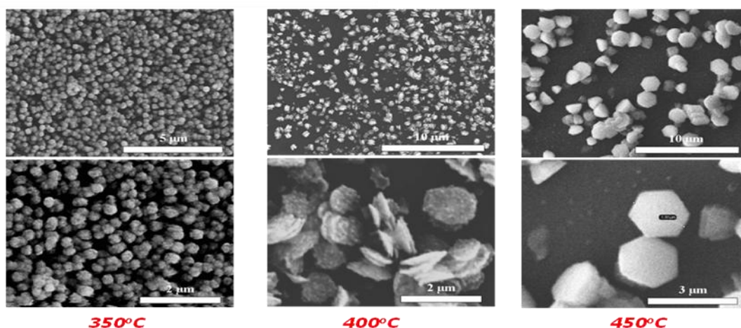
SEM images of ZnO thin films obtained using AACVD of \text{ZnCl}_2(\text{cinnamsczH})_2
